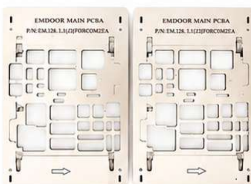
SMT Carrier
